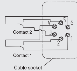
Electrical connection diagram
