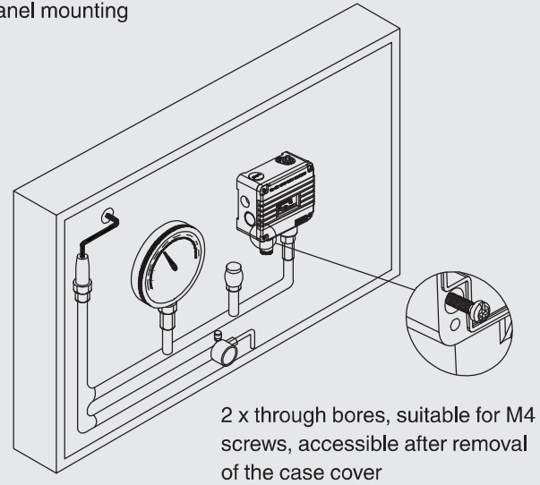
Panel mounting
