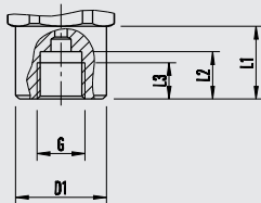
EN 837, female thread, Ermeto-compatible
