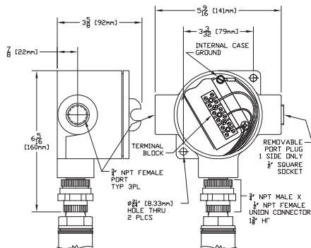
OPTION M513 JUNCTION BOX
