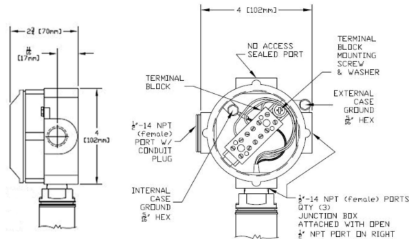
OPTION M460 EXTERNAL GROUNDING SCREW
