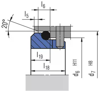
G16 (EN 12756, but l_{lk} is shorter than specified)
