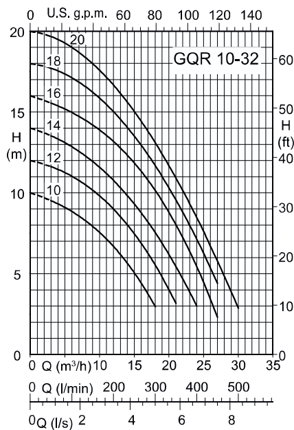
Coverage chart n \approx 2900 rpm
