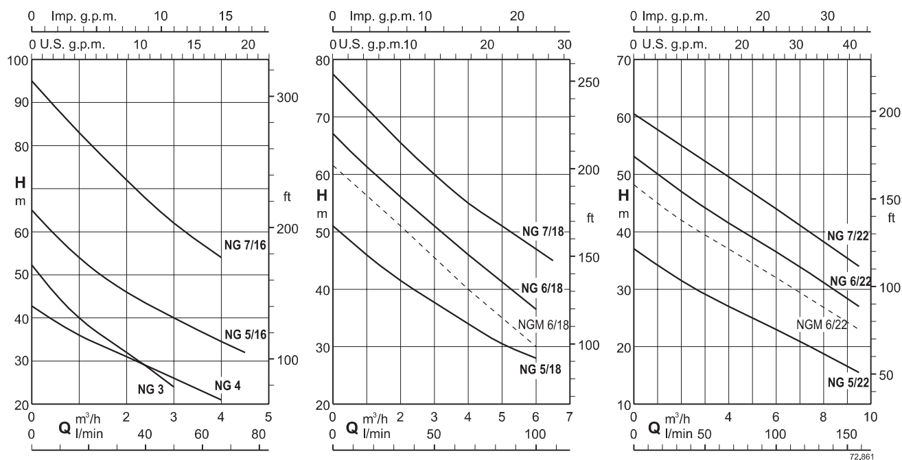
Coverage chart n \approx 2900 rpm
