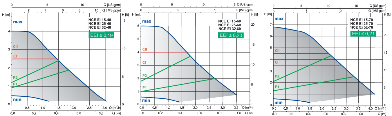
Coverage chart n \approx 2900 rpm
