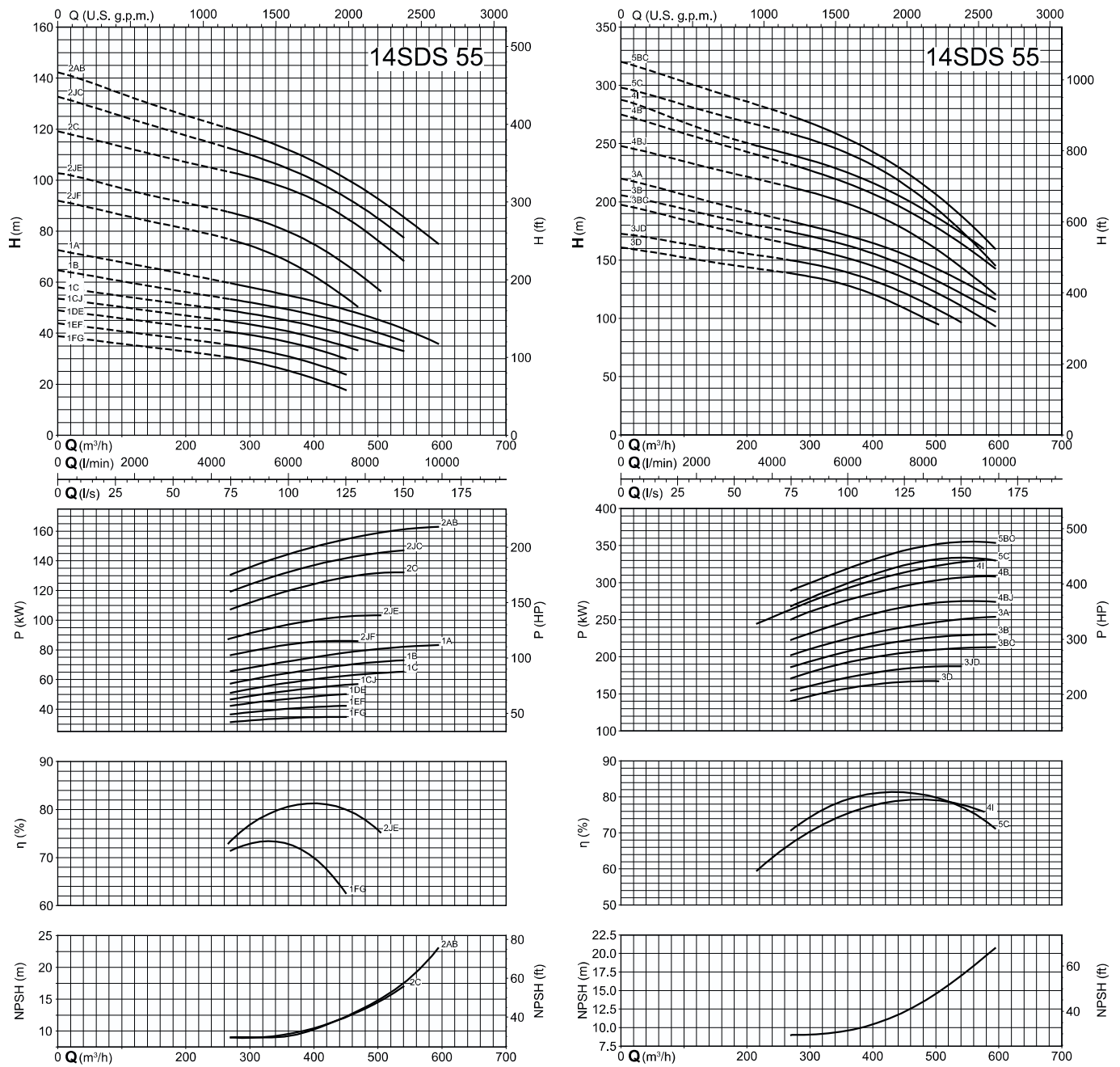
Coverage chart n \approx 2900 rpm
