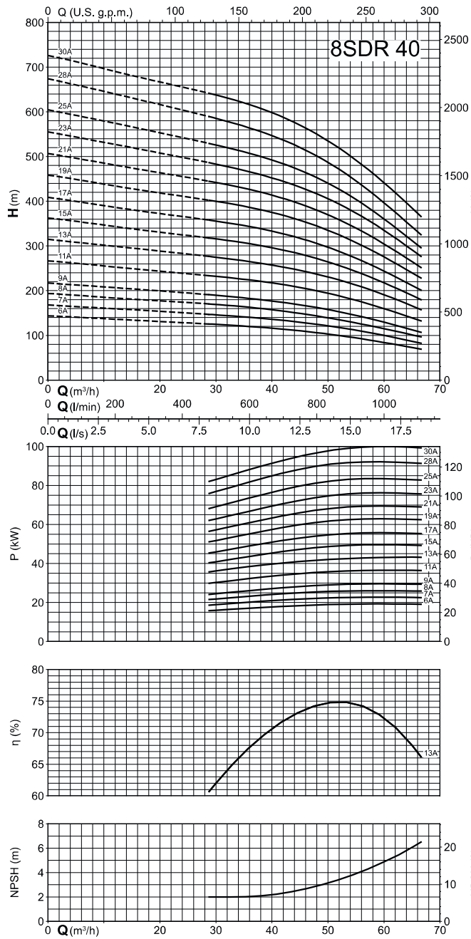
Coverage chart n \approx 2900 rpm
