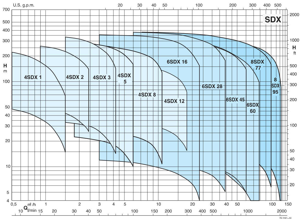
Coverage chart n \approx 2900 rpm
