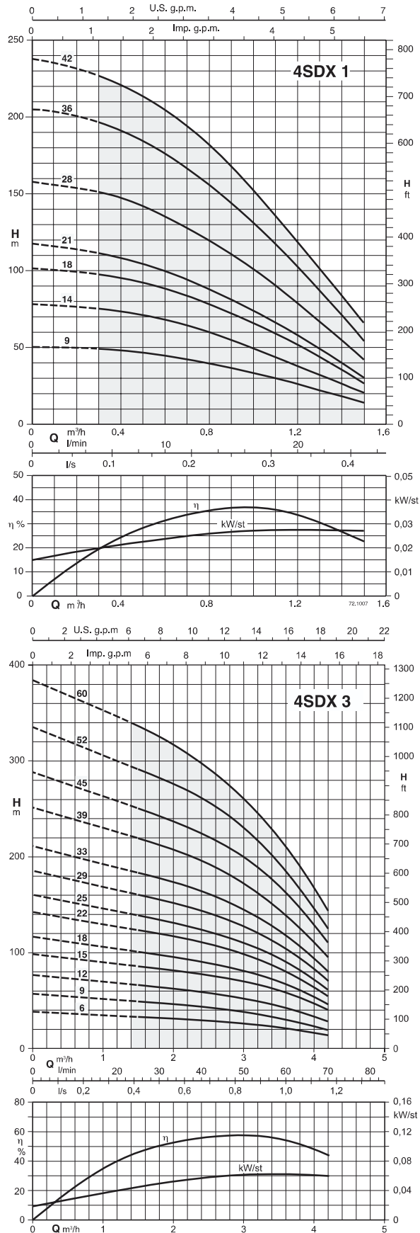
Coverage chart n \approx 2900 rpm
