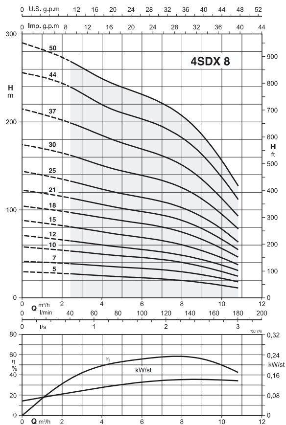
Coverage chart n \approx 2900 rpm
