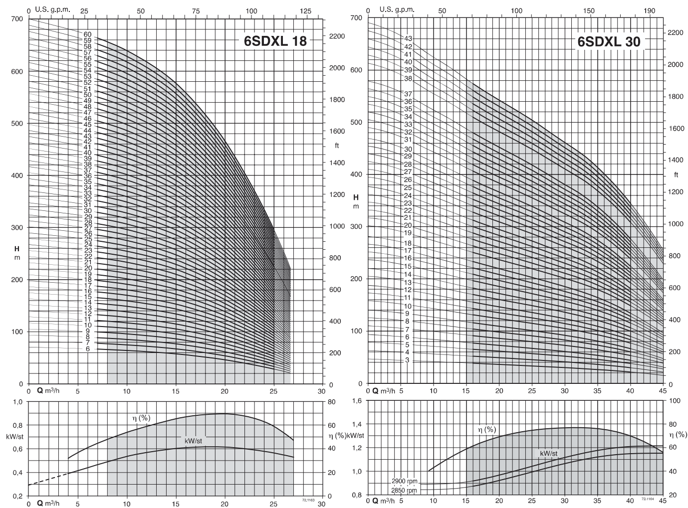
Coverage chart n \approx 2900 rpm
