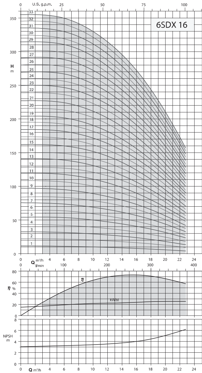
Coverage chart n \approx 2900 rpm
