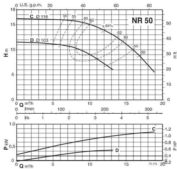
Coverage chart n \approx 2900 rpm
