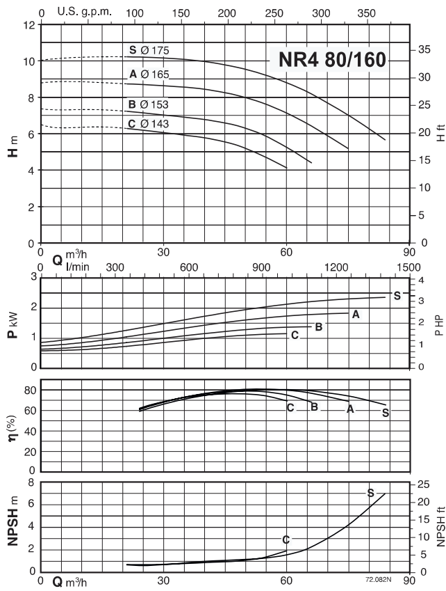
Coverage chart n \approx 1450 rpm
