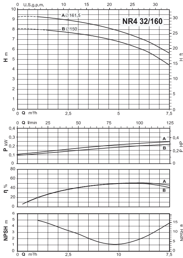
Coverage chart n \approx 1450 rpm
