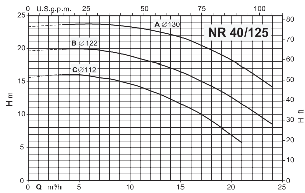
Coverage chart n \approx 2900 rpm
