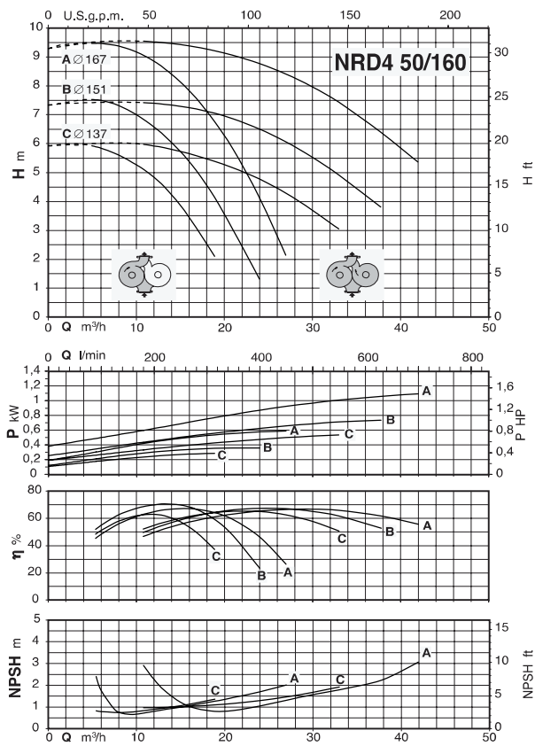
Coverage chart n \approx 1450 rpm
