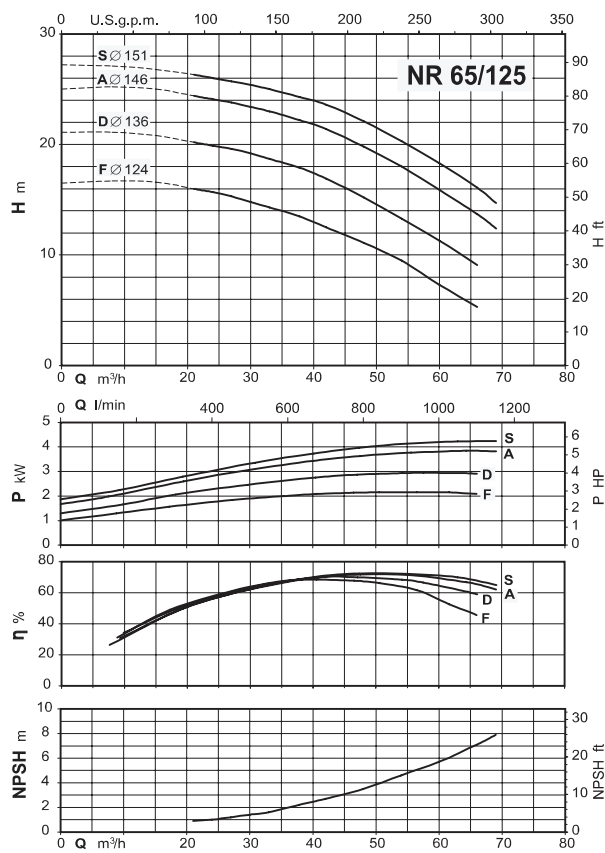
Coverage chart n \approx 2900 rpm
