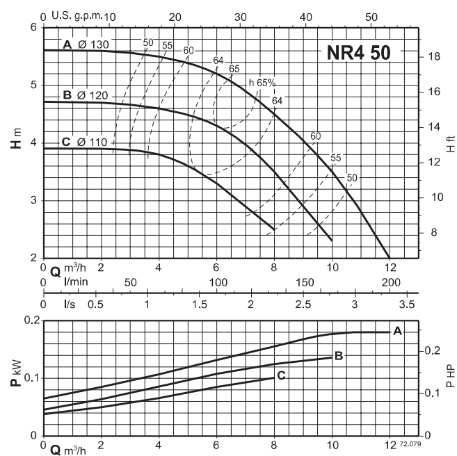
Coverage chart n \approx 1450 rpm
