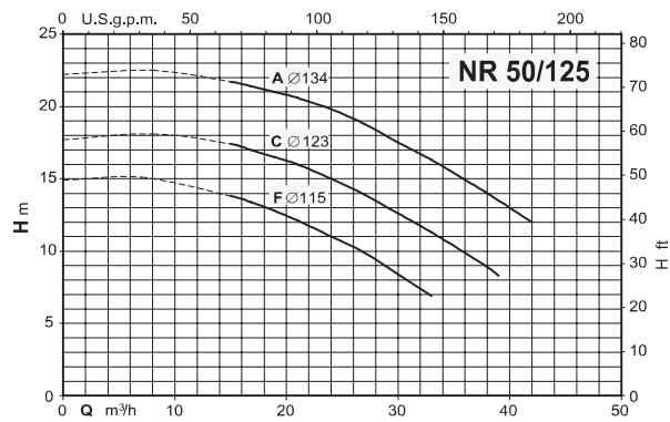
Coverage chart n \approx 2900 rpm
