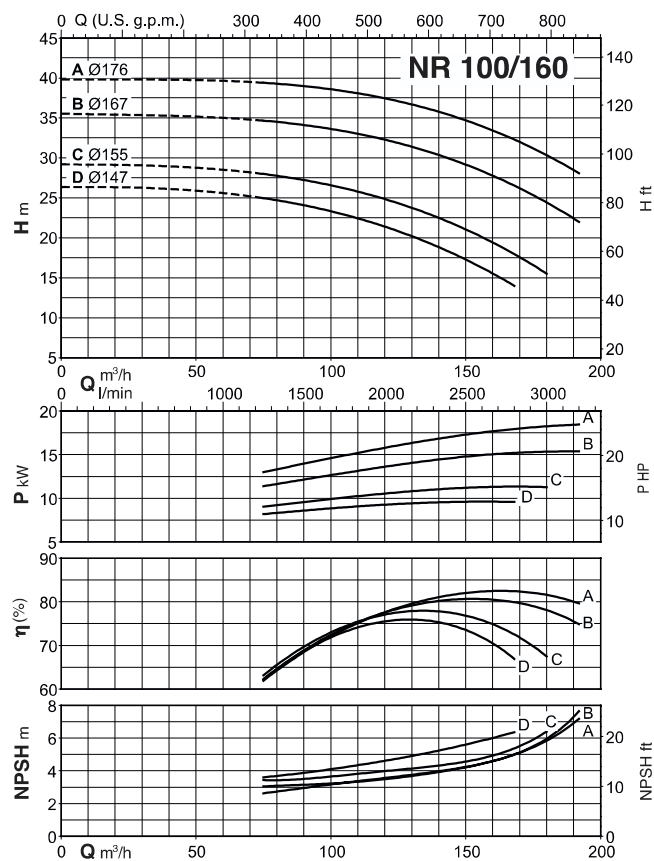
Coverage chart n \approx 2900 rpm
