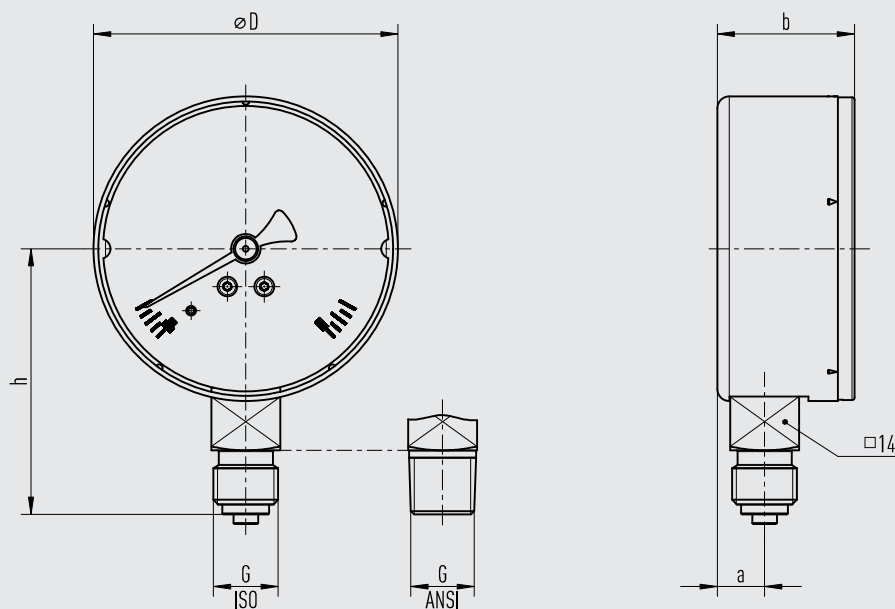
Model 131.11, lower mount (radial)
