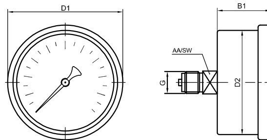
02-Back Connection
