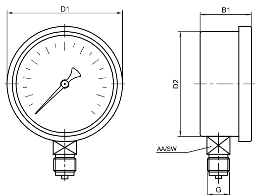
01-Bottom Connection
