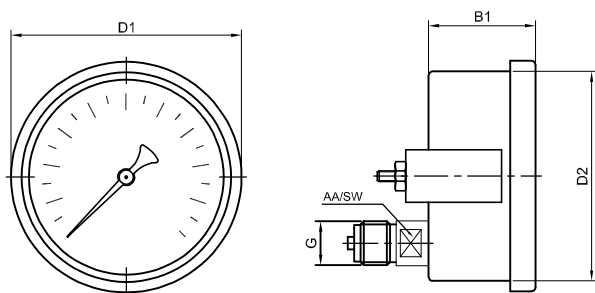
03-Lower Back Panel Mount
