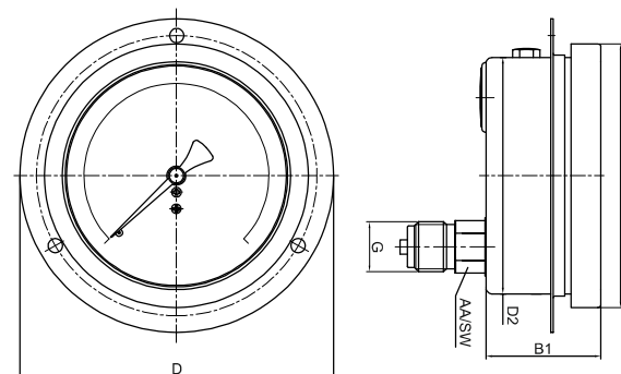
04-Lower Back Front Flange
