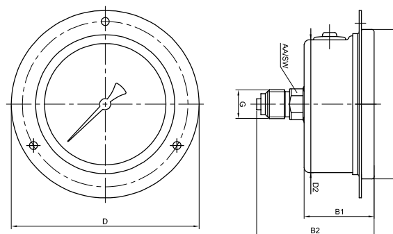
04-Back Connection Front Flange
