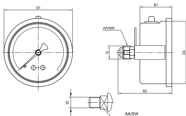
03-Back Connection Panel Mount
