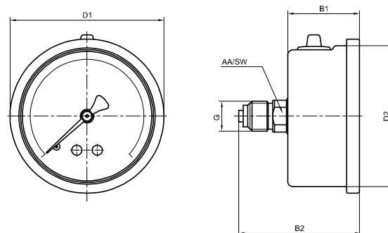
02-Back Connection
