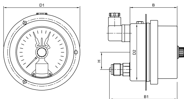
04-Lower Back, Front Flange Connection
