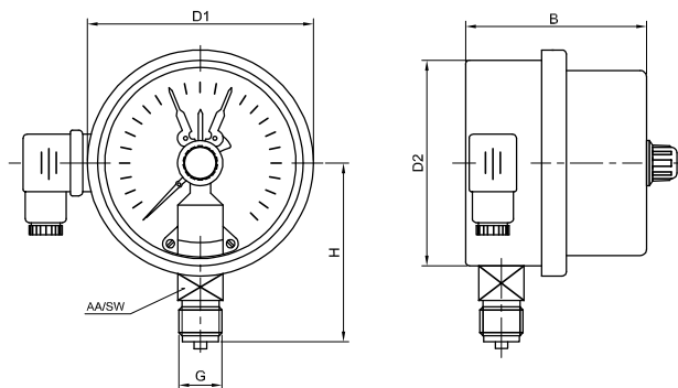
01-Bottom Connection
