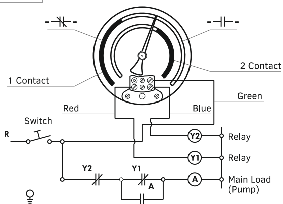
NCNO
