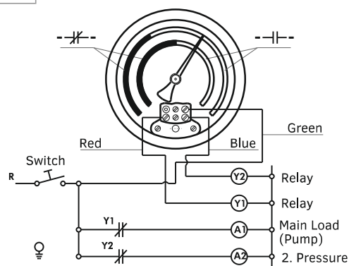
NCNC
