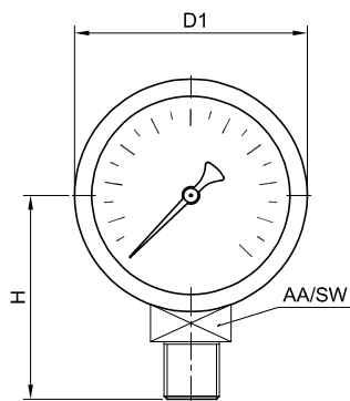
01-Bottom Connection
