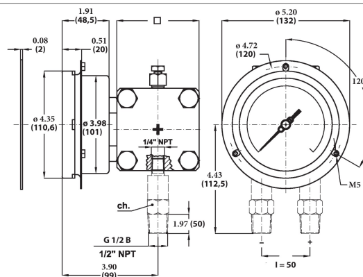
Lower (Mounting code A ) , with front flange (Option code F ): DS 4" (100mm)
