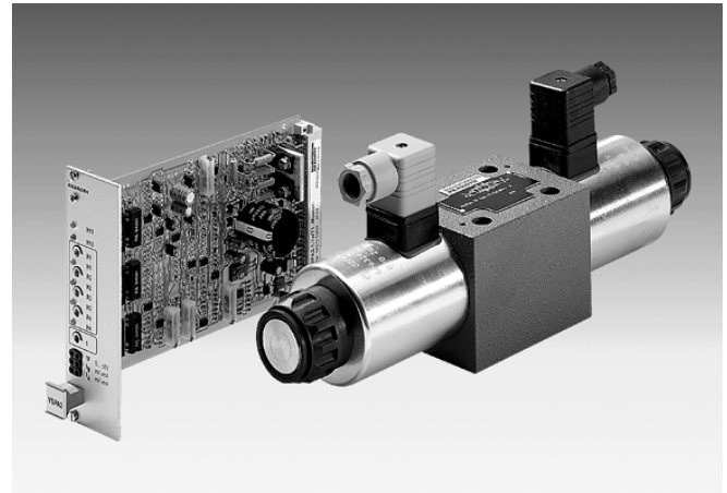
Type 4WRA 10 ...-2X/G24...K4/.V with plug-in connectors and associated control electronics (separate order)
