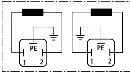
Connection on component plug
