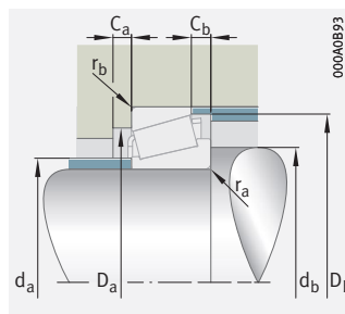
Mounting dimensions
