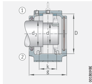
Double lip seal EDH, cover
