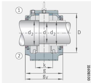
V-ring seal EDV
