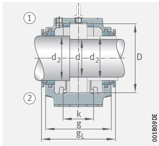
Labyrinth seal ETS
