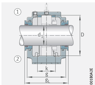
Labyrinth seal ETS
